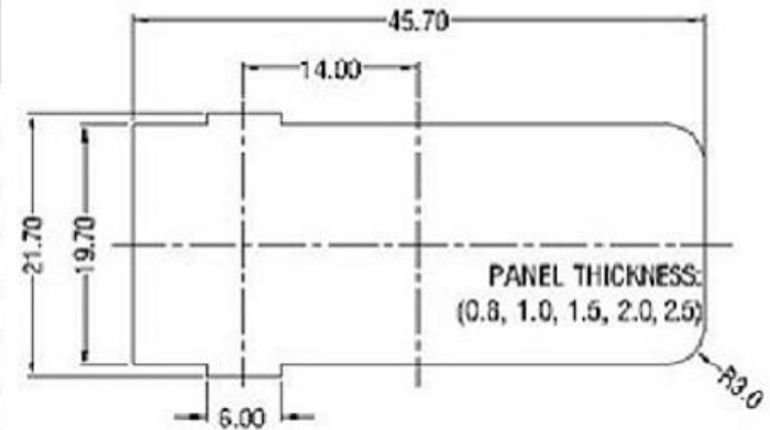
PANEL CUT-OUT
